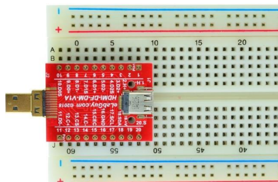
Figure 2: Example of connecting the HDMI-DF-DM-V1A on a proto PCB (Note: This picture only shows the pins spacing, actual use may not be used on a breadboard)
