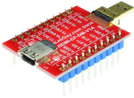
Figure 3: HDMI-DF-DM-V1A with headers
