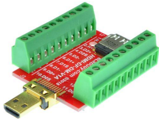
Figure 4: HDMI-DF-DM-V1A with terminal blocks
