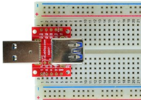
Figure 2: Example of connecting the USB3-AM-AF-V1A on a breadboard (Note: This picture only shows the pins spacing, actual use may not be used on a breadboard)
