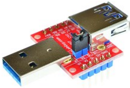
Figure 3: USB3-AM-AF-V1A with headers
