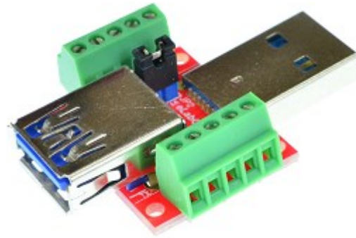
Figure 4: USB3-AM-AF-V1A with terminal blocks
