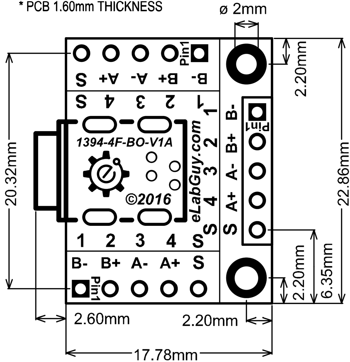
PCB outline Drawing
