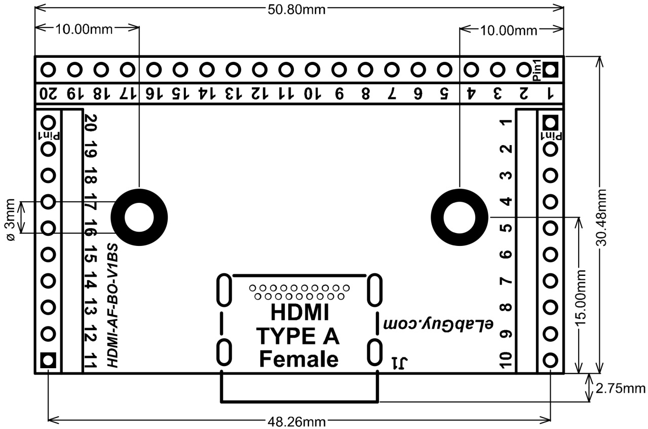
HDMI-AF-BO-V1BS Schematic Diagram
