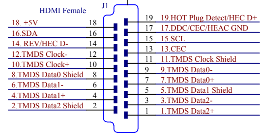
HDMI-AF-BO-V1BS Schematic Diagram
