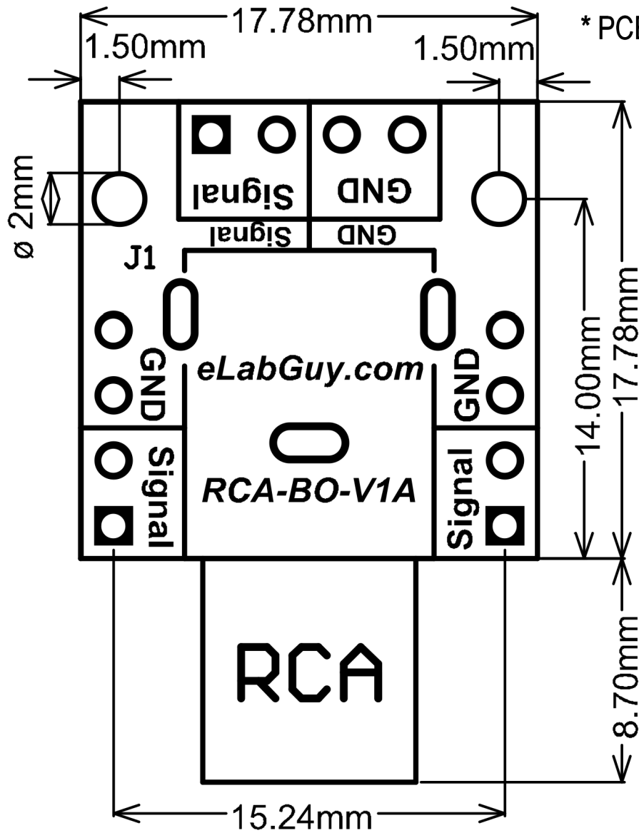
RCA-BO-V1A PCB outline Drawing
