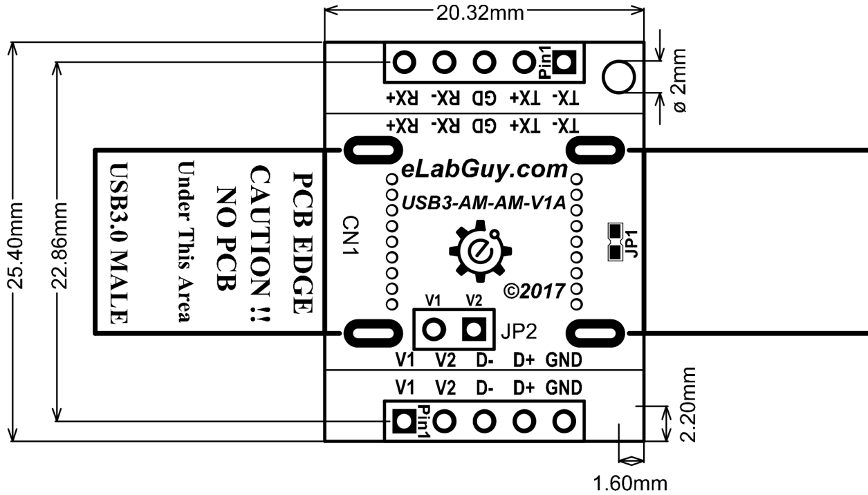
Header 2X1 _2.54mm
