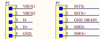
Header 5X1 _2.54mm
